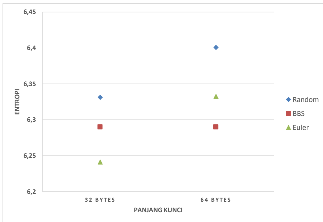
Gambar 3. Nilai Entropi Hasil Preliminary Experiment
